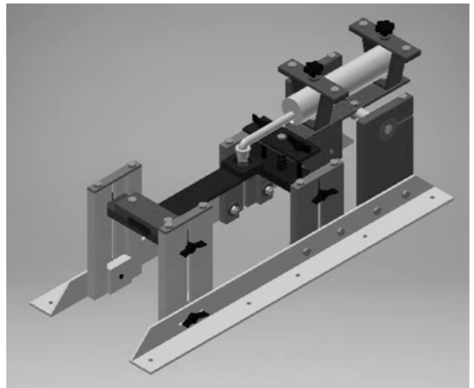
FIGURE 1. Computer-aided design of the tooth brushing simulation device
